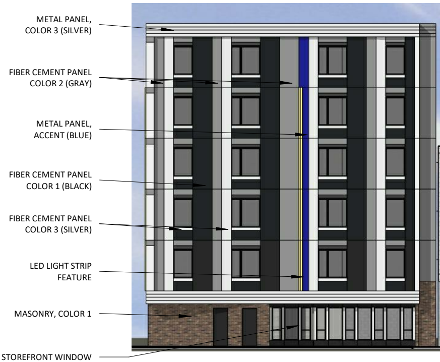
1 212 STATE - CONCEPT - EAST ELEVATION FP5.2 1" = 20'-0"
