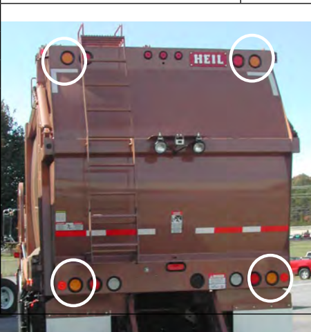
Peterson Multi-Function Lights LED Strobes & Turn Light Combination
