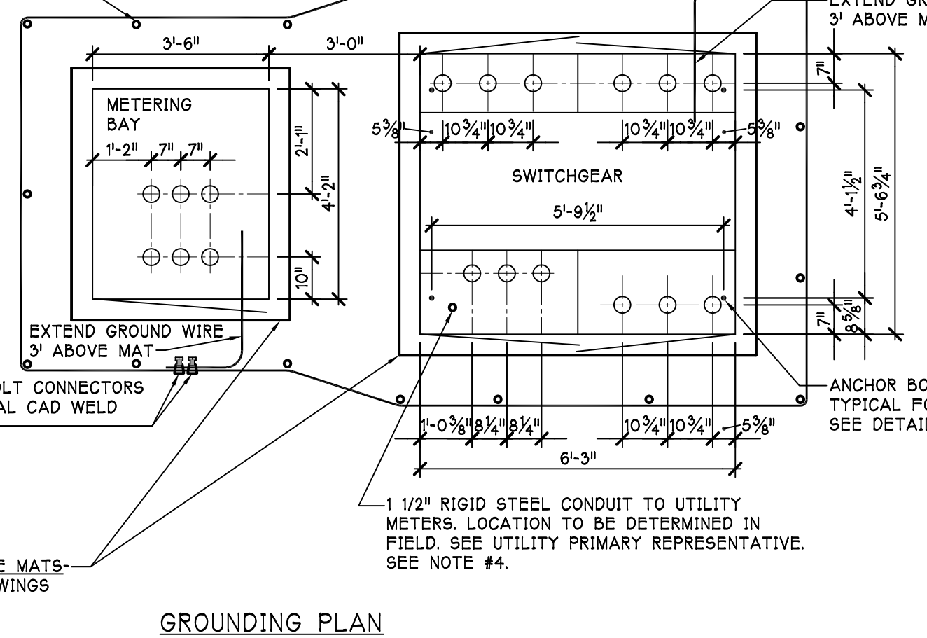
GROUNDING PLAN
