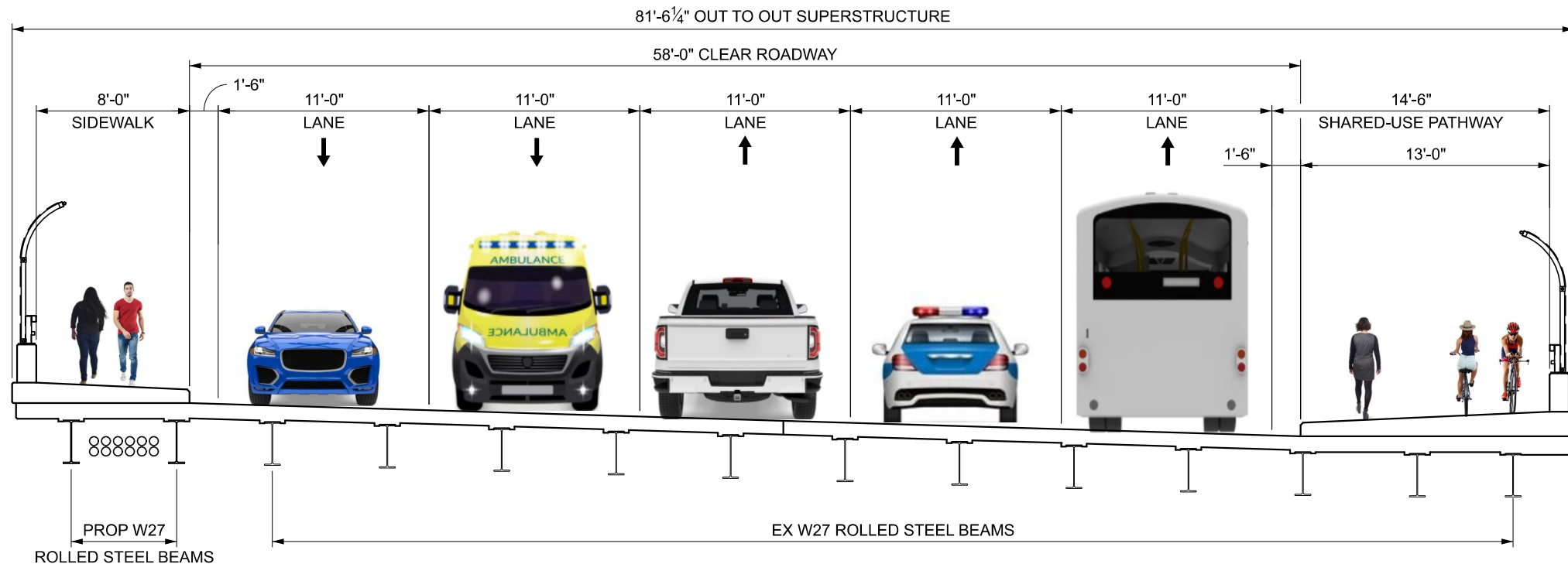
PROPOSED SECTION (LOOKING NORTH)
