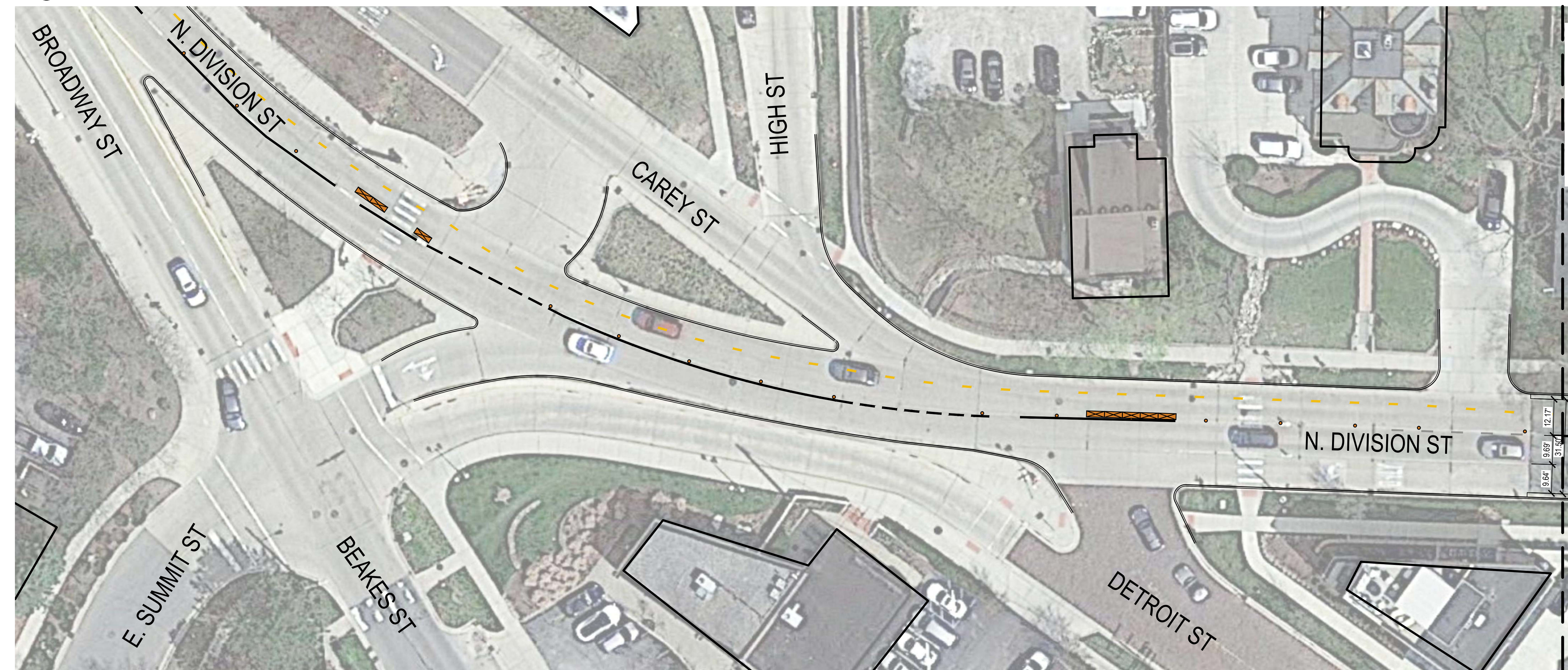
8 PROPOSED S. DIVISION ST 8 SCALE: 1" = 20'
