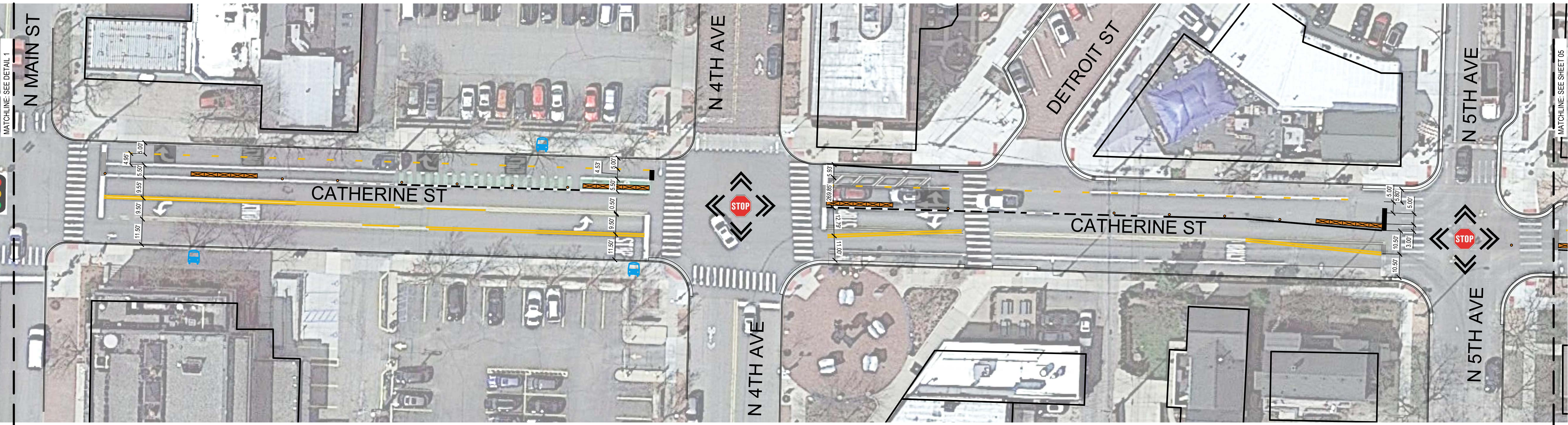
2 PROPOSED MILLER - CATHERINE 2 SCALE: 1" = 20'
