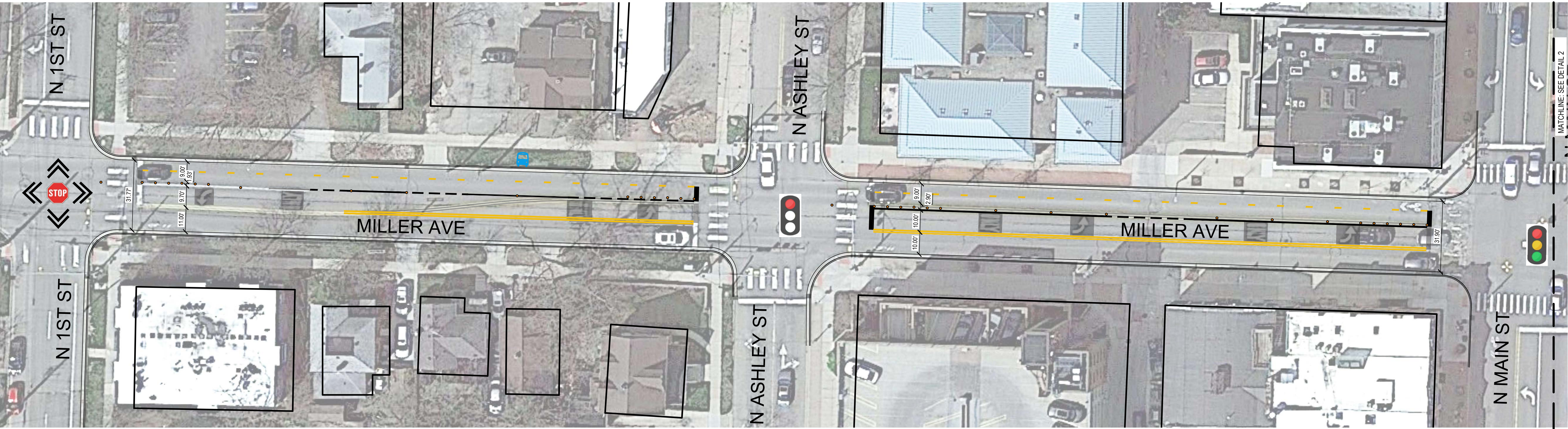
1 PROPOSED MILLER - CATHERINE 1 SCALE: 1" = 20'
