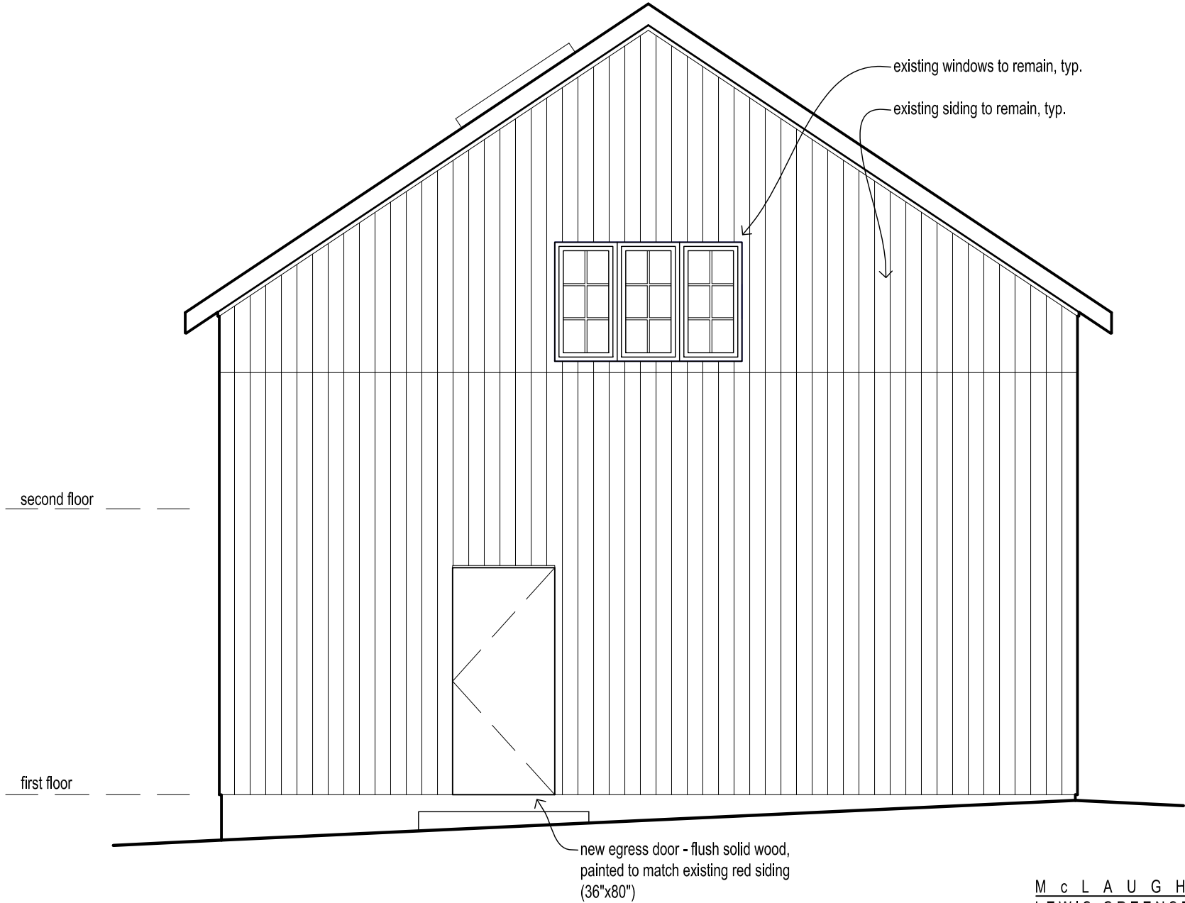
REAR ELEVATION
