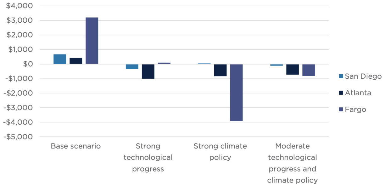
Figure 8: Relative net present value of lifetime costs for ASHPs versus furnace and air conditioner combinations, across the base case and three technology and policy scenarios
