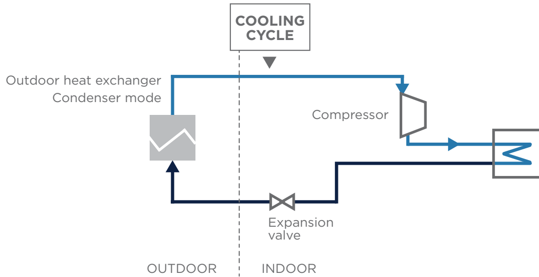
Figure 3: The cooling cycle of an ASHP
