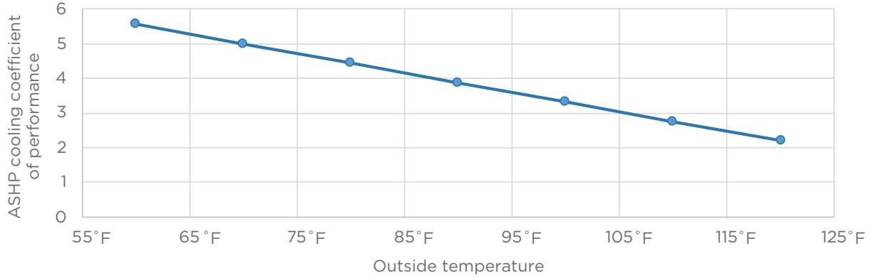
Figure 10: ASHP cooling performance
