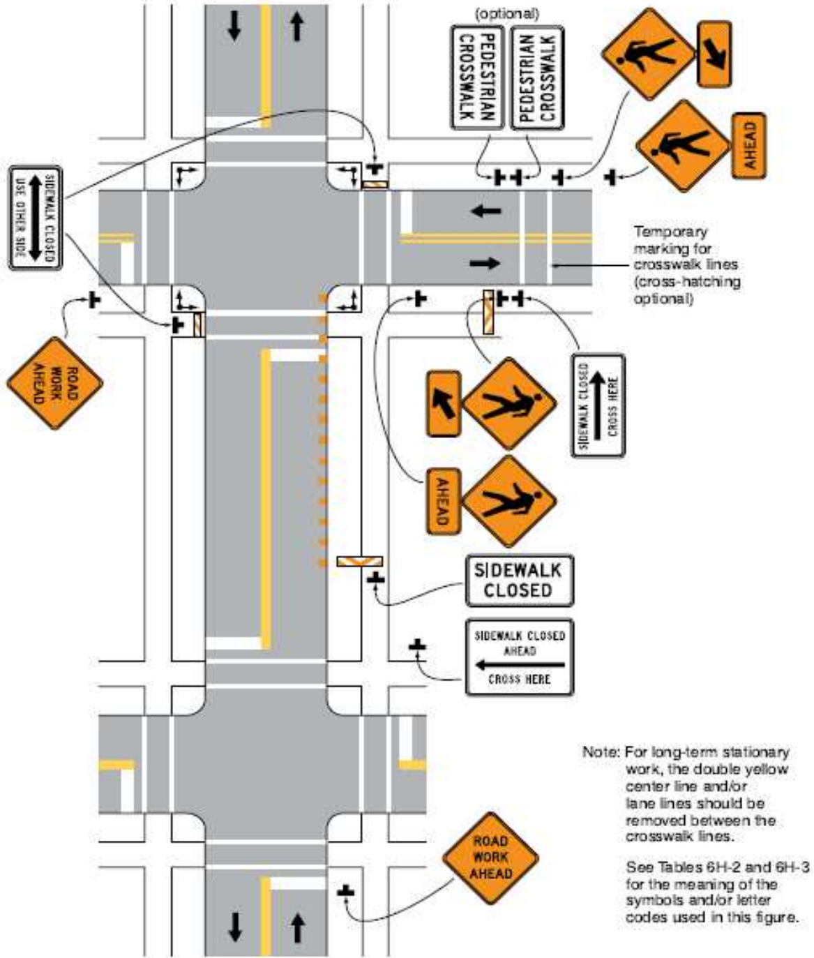
Typical Application 29
