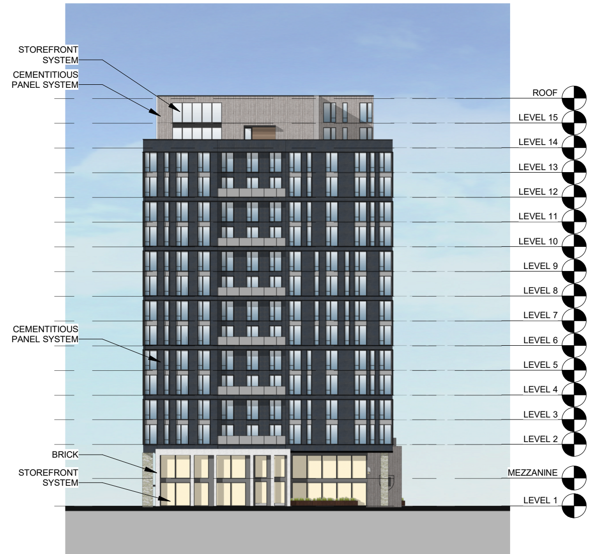
1 SOUTH ELEVATION
