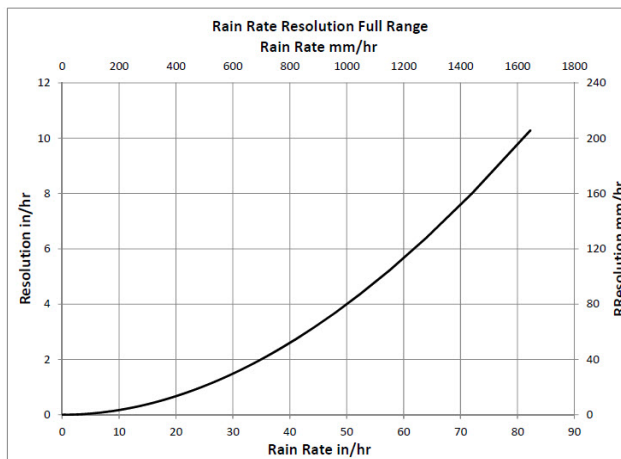
Figure 2. Full Range Rain Rate Resolution
