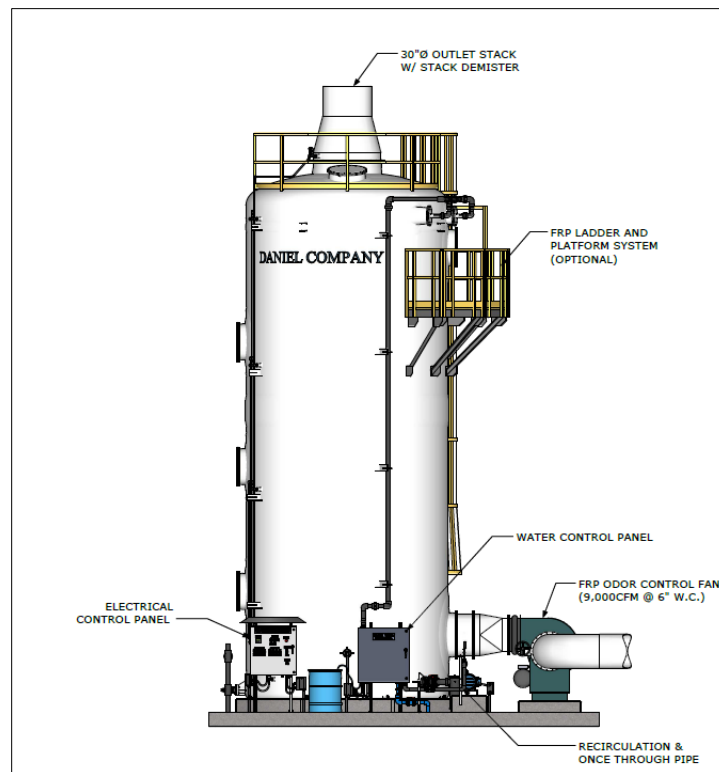
Figure 5-10. Biotower Layout
