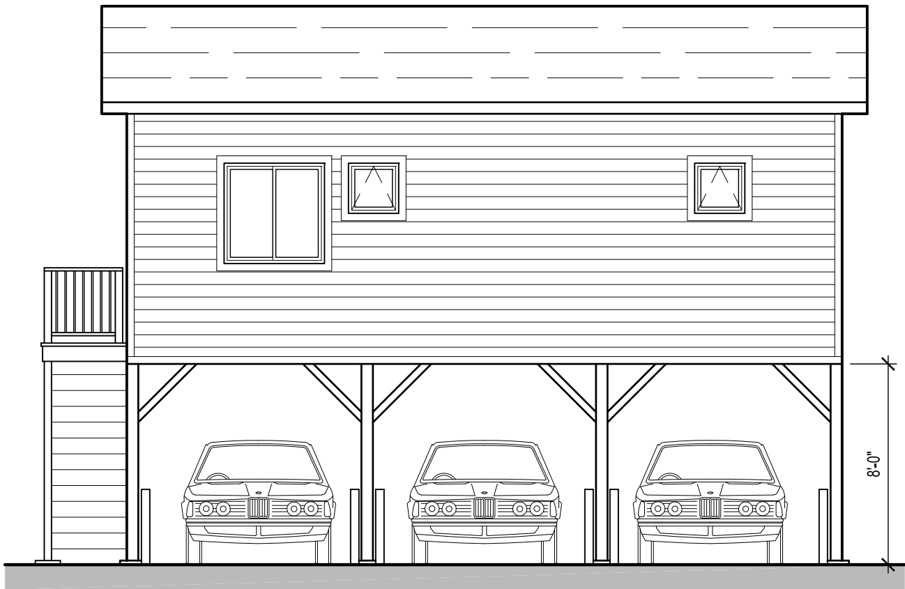
NORTH ELEVATION
