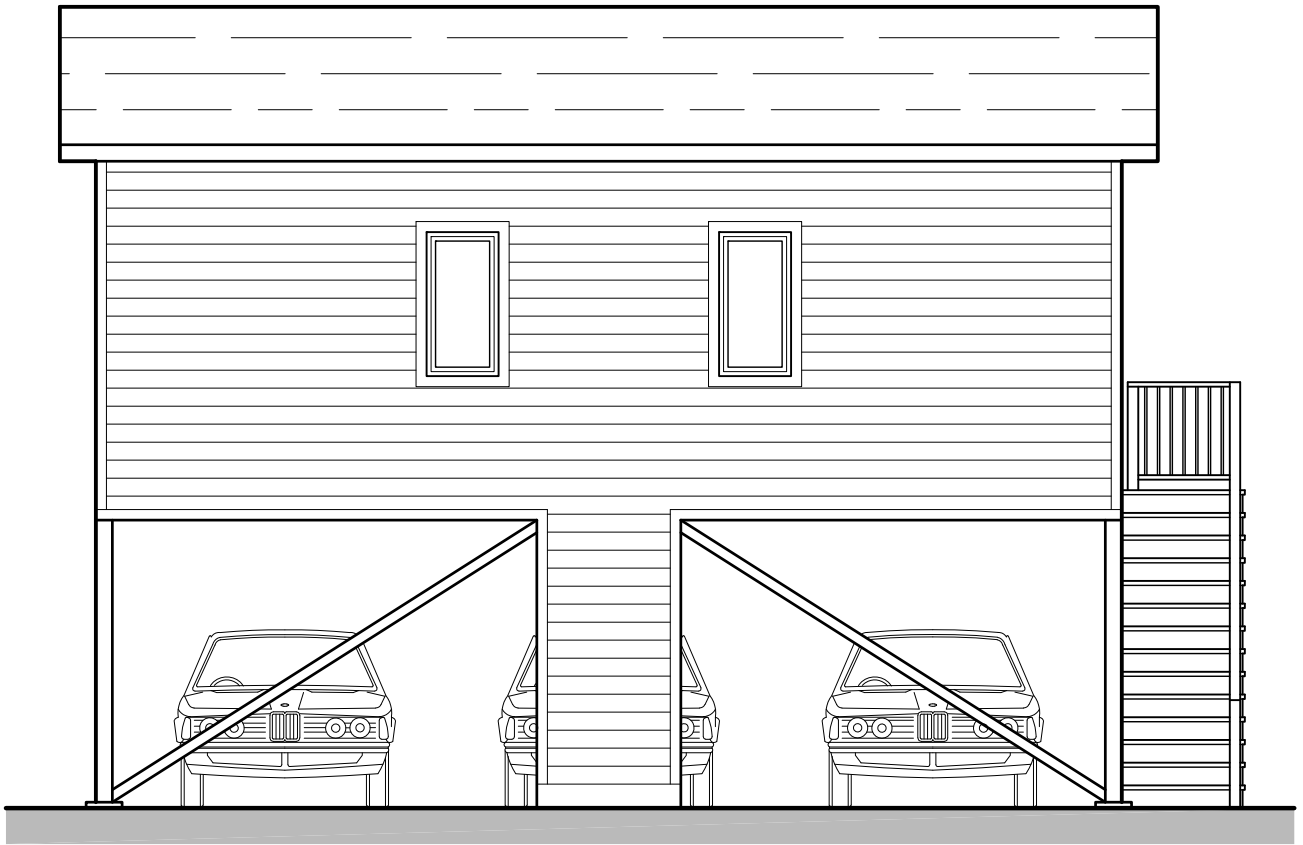
SOUTH ELEVATION
