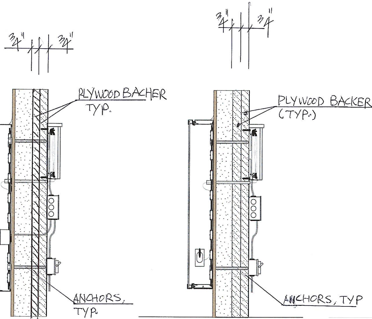
Typical Floret Construction and Mounting Detail
