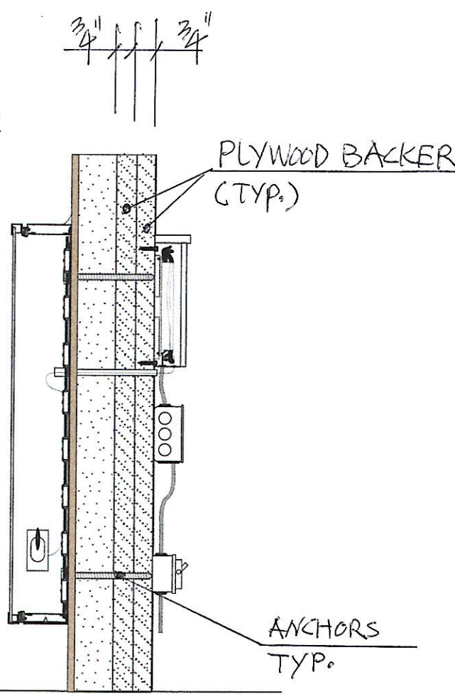
Typical Floret Construction and Mounting Detail
