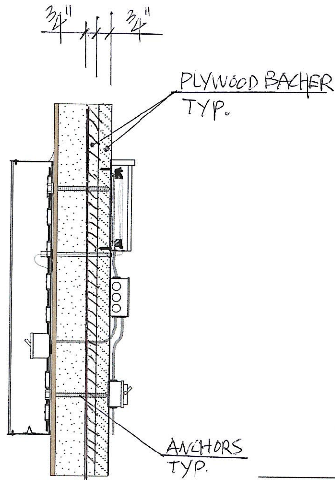
Typical Floret Construction and Mounting Detail
