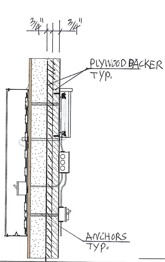
Typical Channel Letter Construction and Mounting Detail
