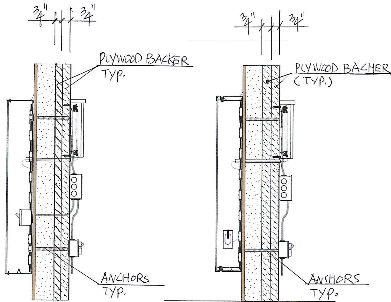
Typical Floret Construction and Mounting Detail
