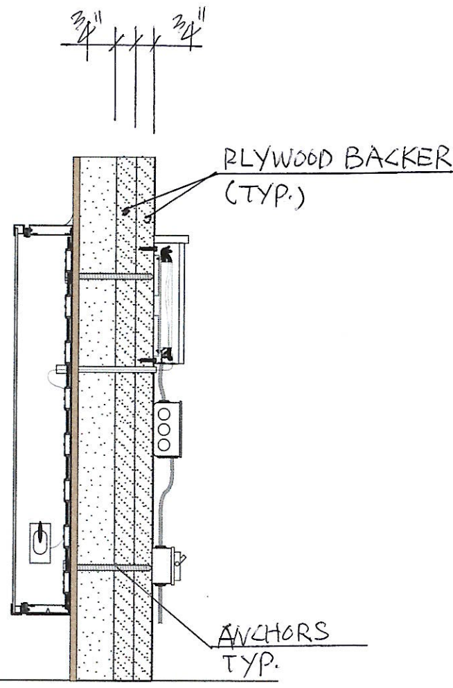
Typical Floret Construction and Mounting Detail
