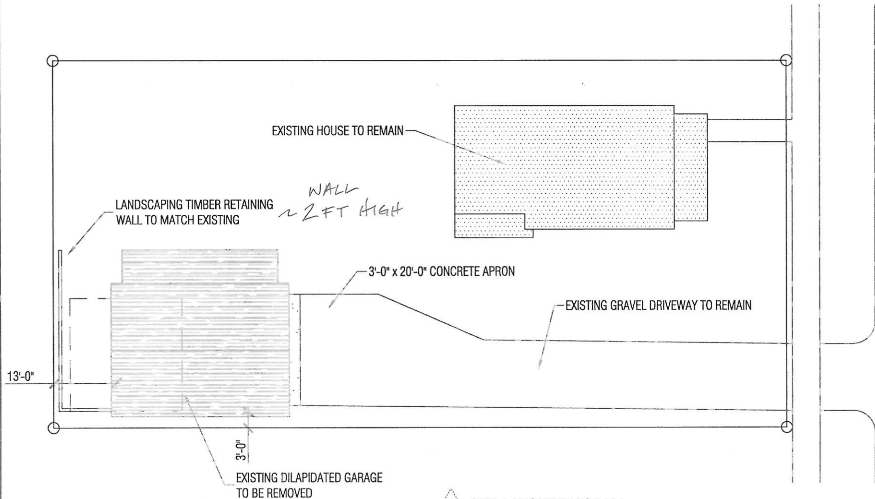
SITE LAYOUT DIAGRAM
