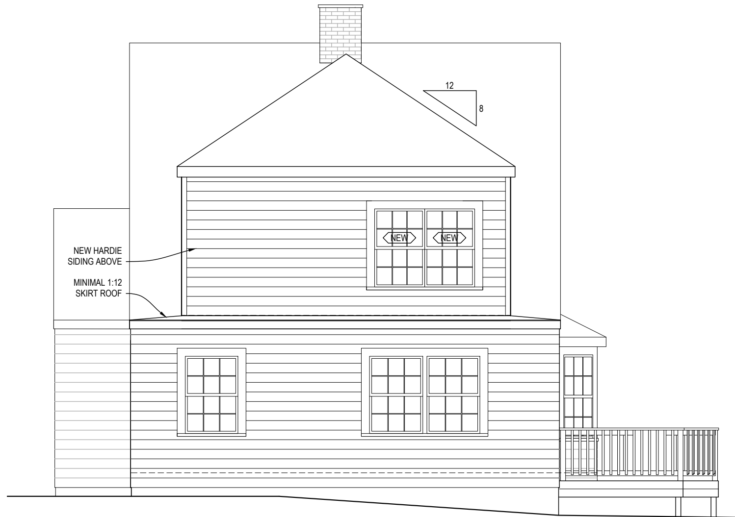
WEST ELEVATION
