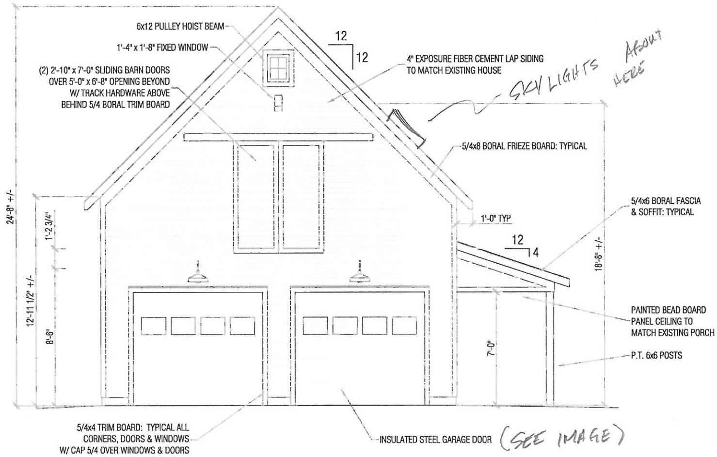
④ EAST ELEVATION Scale: 3/16" = 1'-0"
