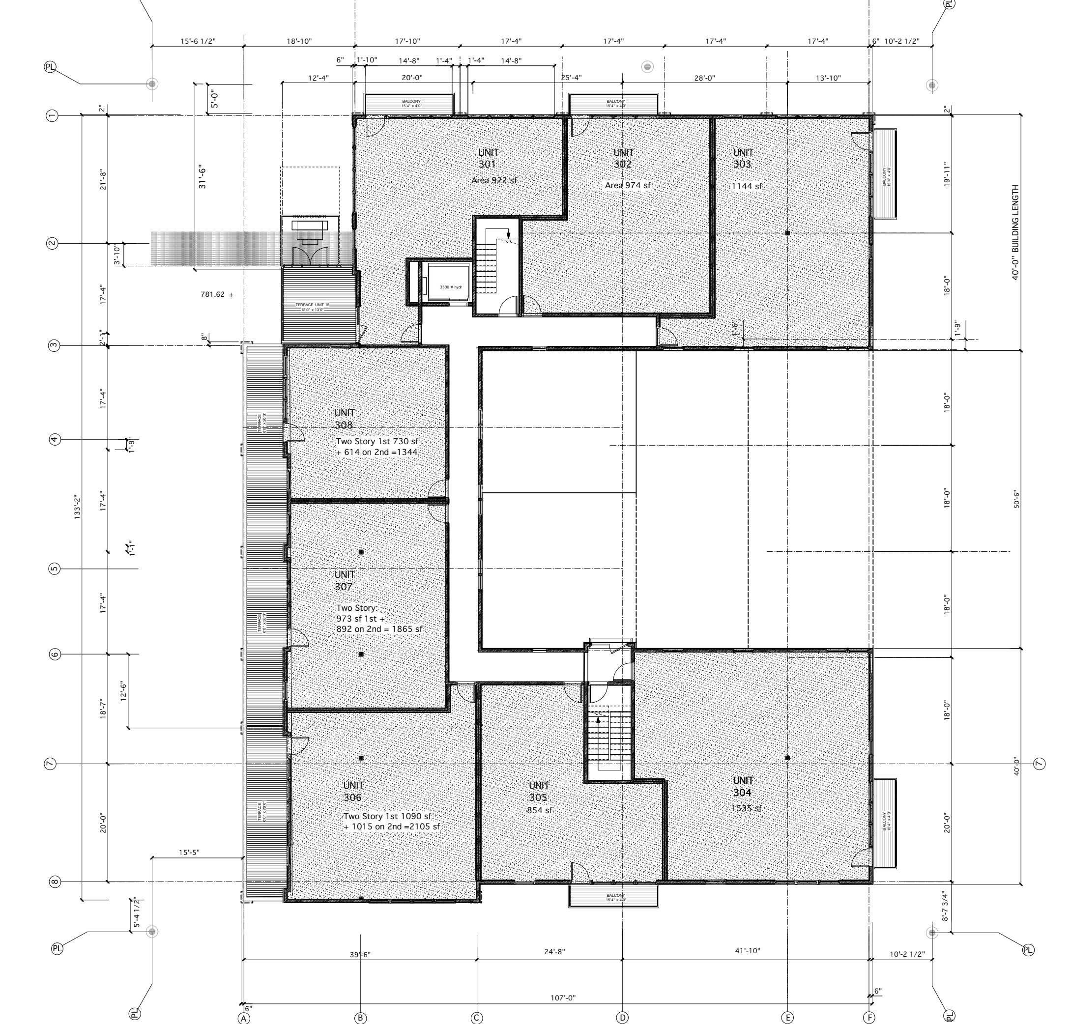
THIRD FLOOR Scale: 1/16" = 1'-0" on 24" x 36"
