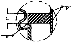
DETAIL A STEEL ASSEMBLY DETAIL N.T.S.
