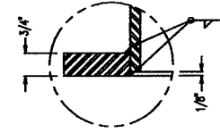
DETAIL B STEEL ASSEMBLY DETAIL N.T.S.
