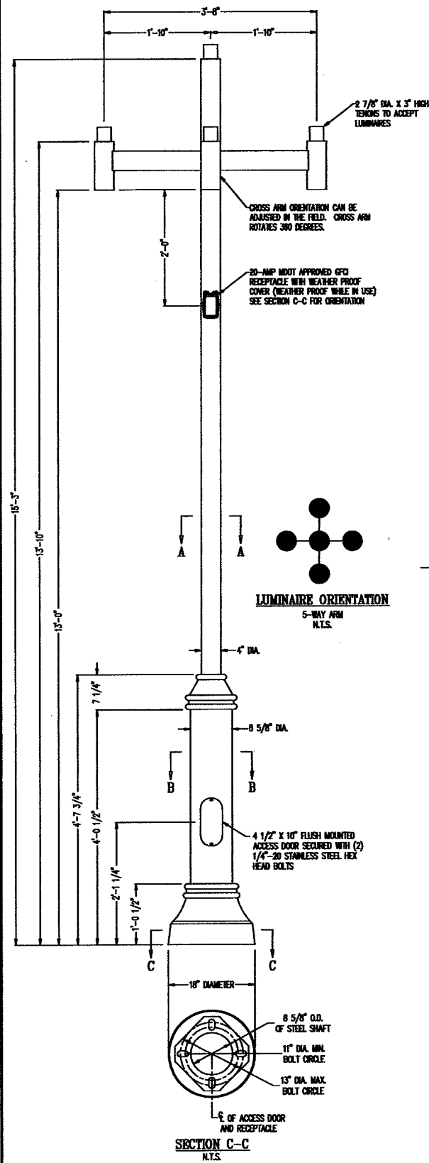
DETAIL A STEEL ASSEMBLY DETAIL N.T.S.
