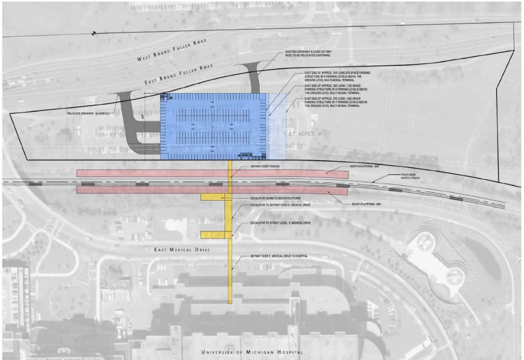
ANN ARBOR MULTI-MODAL TRANSIT CENTER FIGURE 2 - PARKING DECK FOOTPRINT
