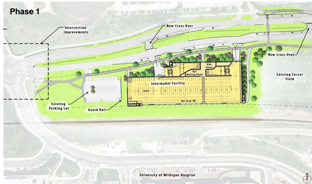
Fuller Road Station: Phase One Concept Plan
