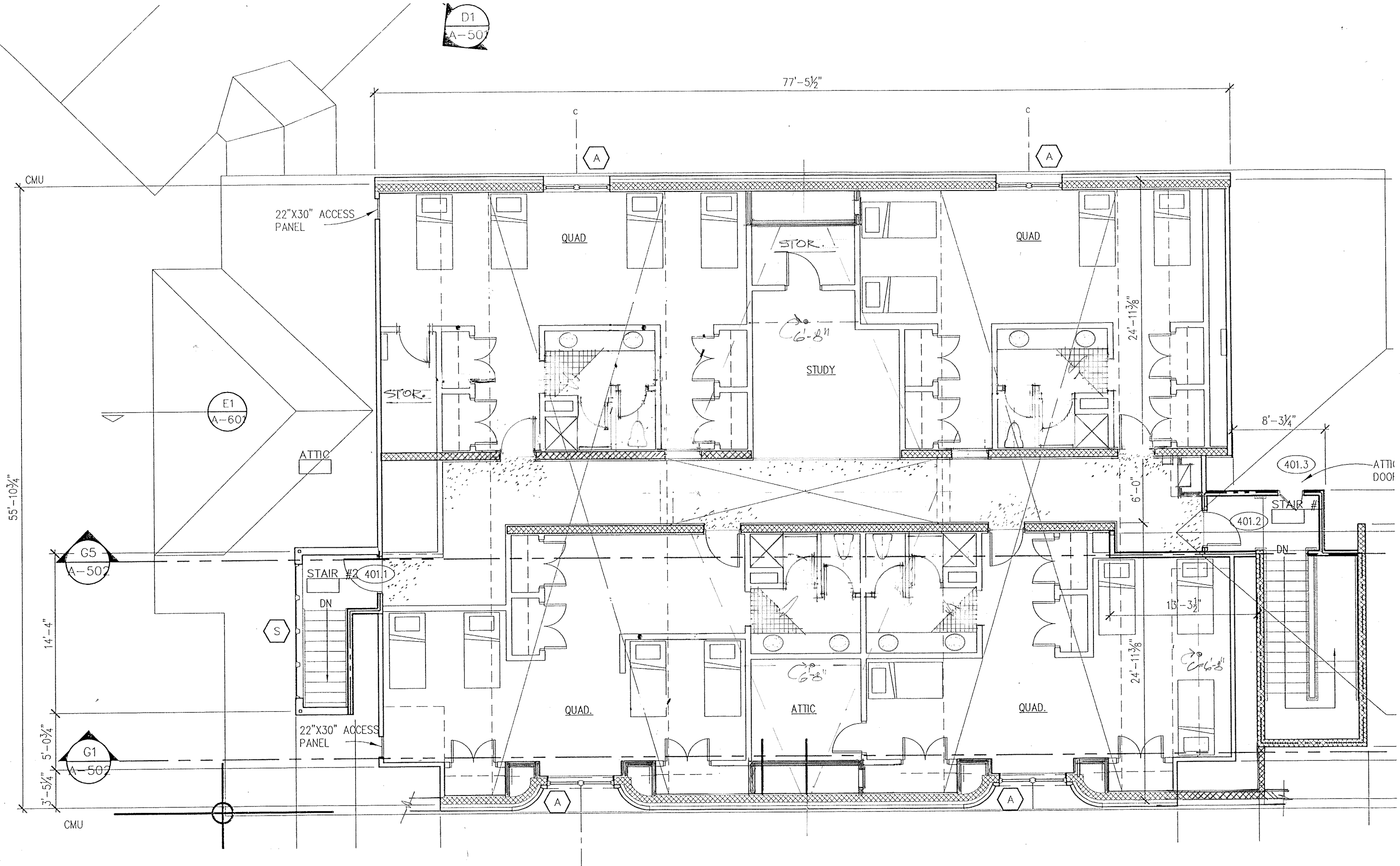
PROPOSED LAYOUT - LOFT AREA
