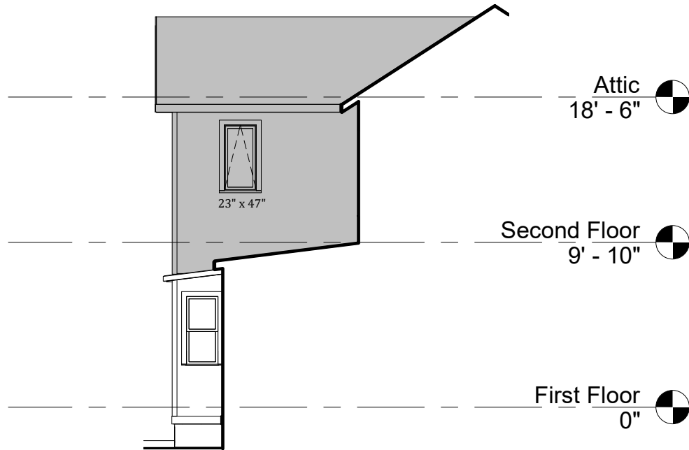
① East Elevation, Addition 1/8" = 1'-0"
