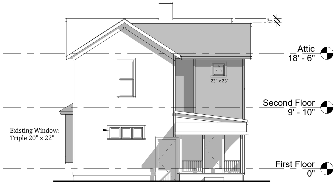
① West Elevation 1/8" = 1'-0"
