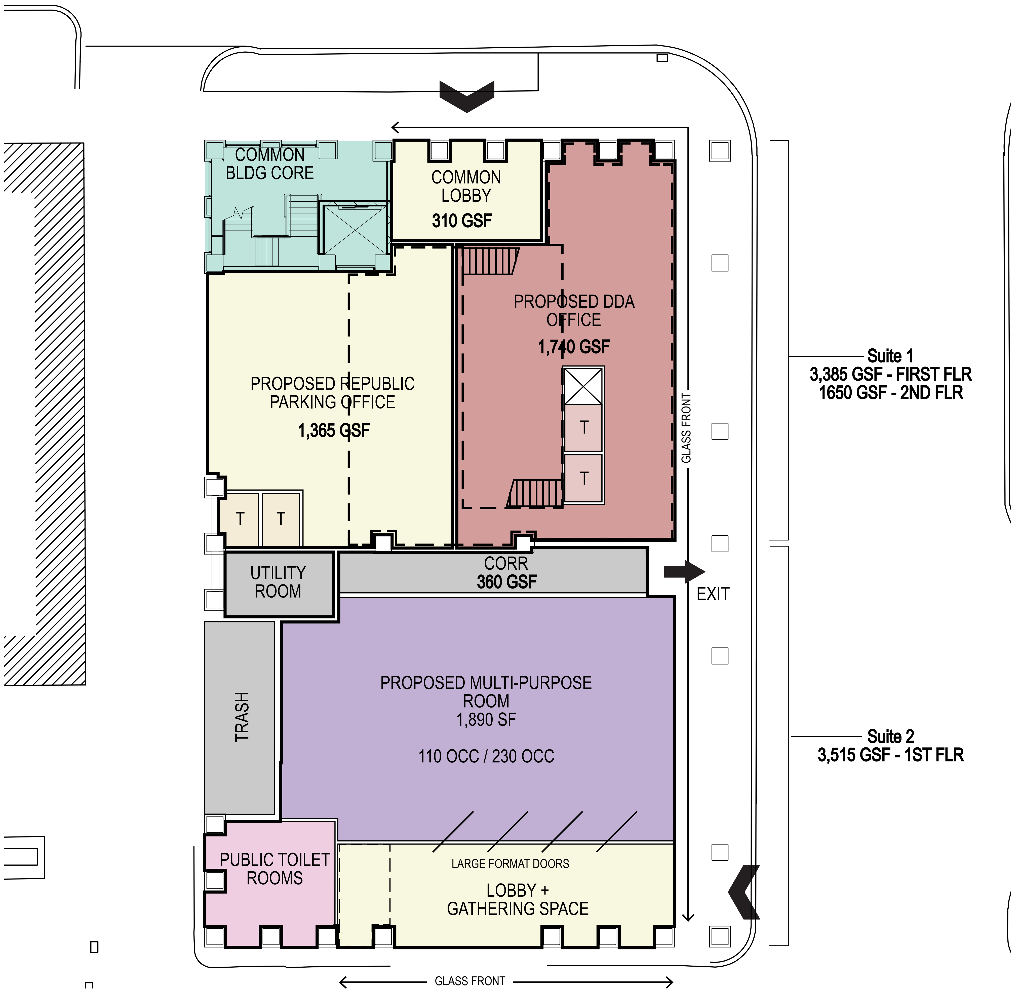
FIRST FLOOR PLAN DIAGRAM NOT TO SCALE
