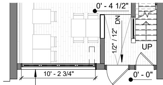
PROPOSED ELEVATION AND PLAN
