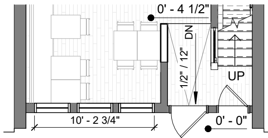
EXISTING ELEVATION AND PLAN
