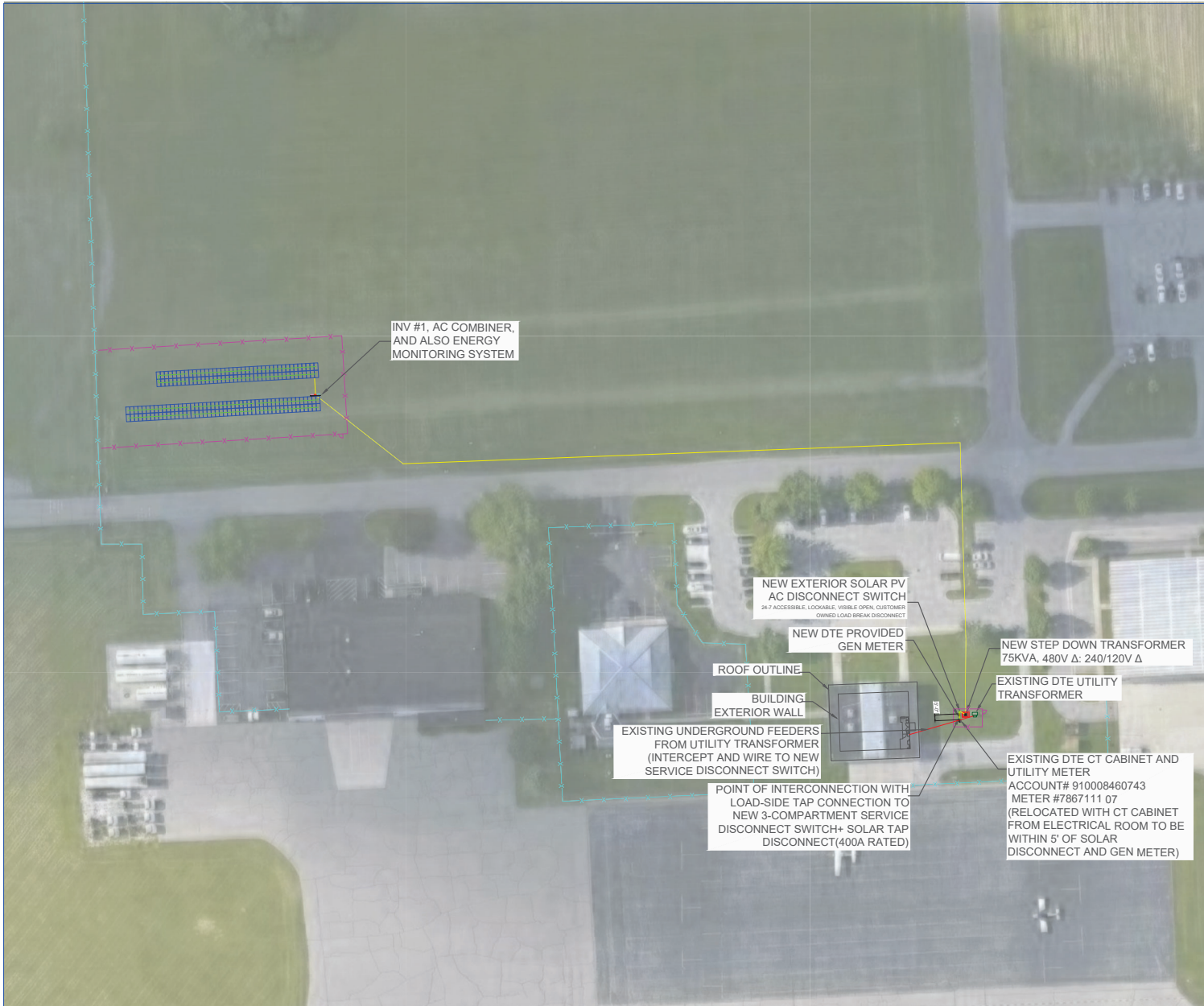
1 SITE PLAN SCALE: 1" = 40' - 0"
