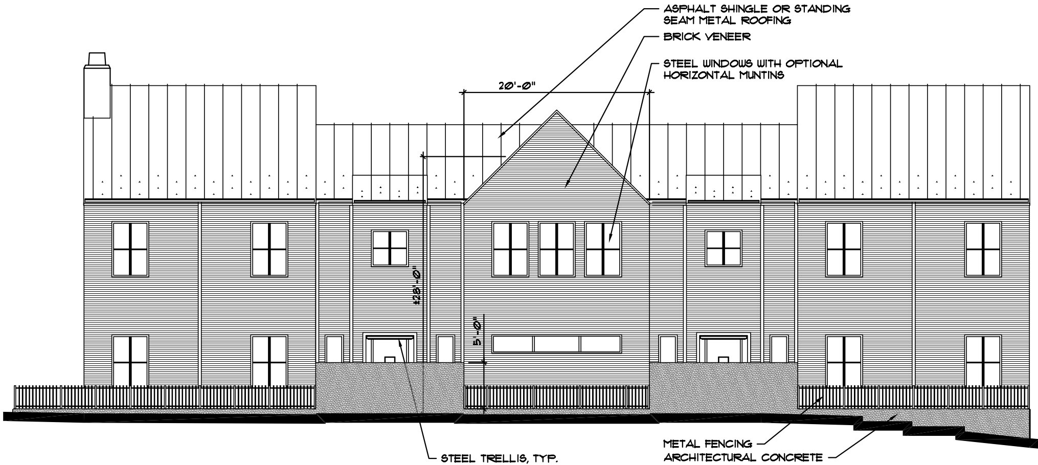
1 SIDE ELEVATION (NORTH) A3.0 SCALE: 3/32" = 1'-0"
