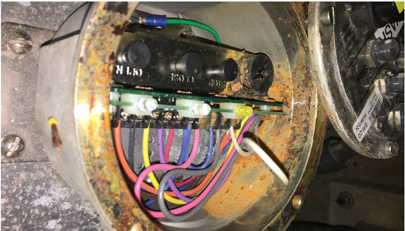
EIM valve actuator remote control station. Device was immersed and is not functioning. Housing and wire terminations are corroding. Typical of 50
