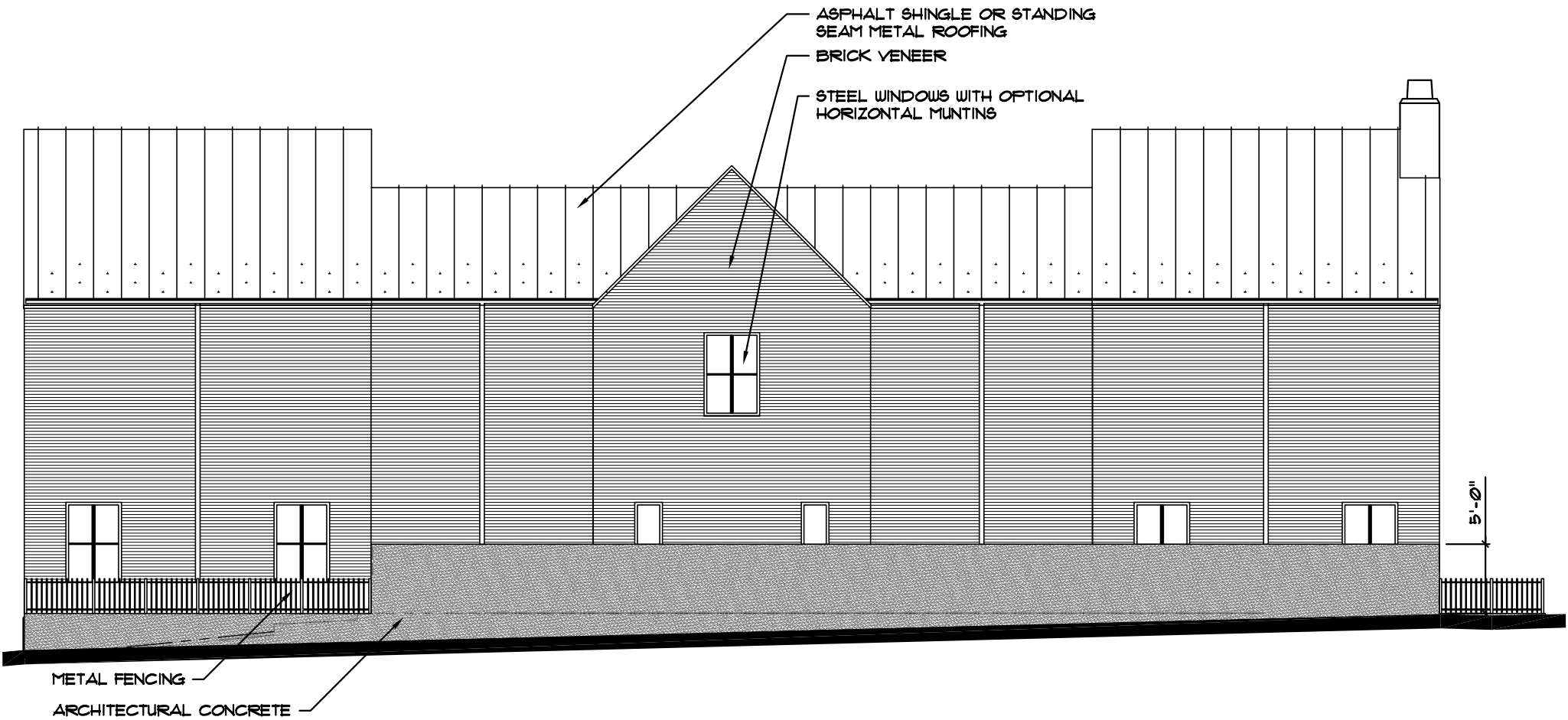
1 SIDE ELEVATION (SOUTH) A4.0 SCALE: 3/32" = 1'-0"
