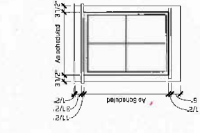
Window Type A
