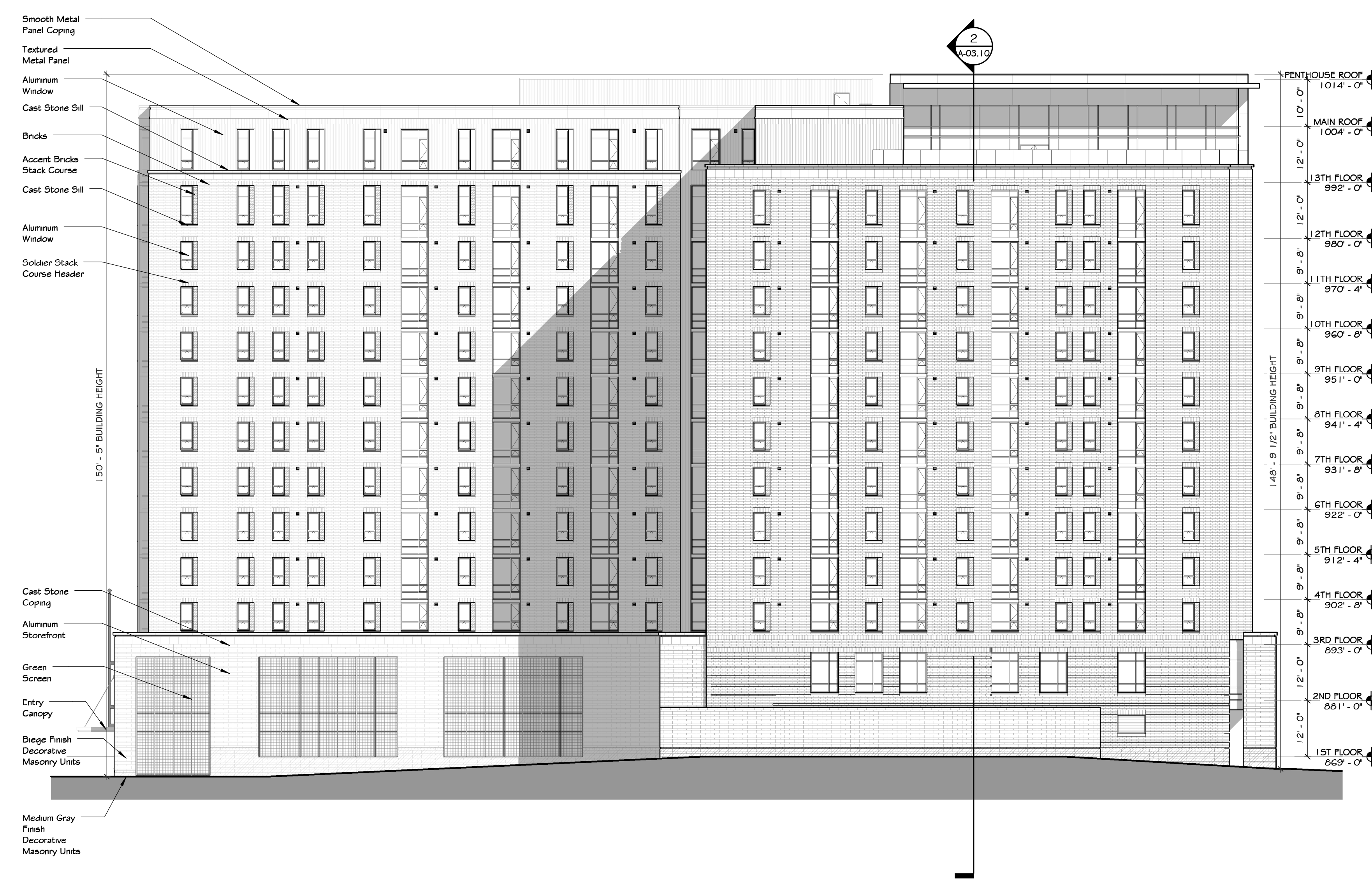
1 West Building Elevation Scale: 1/16" = 1'-0"
