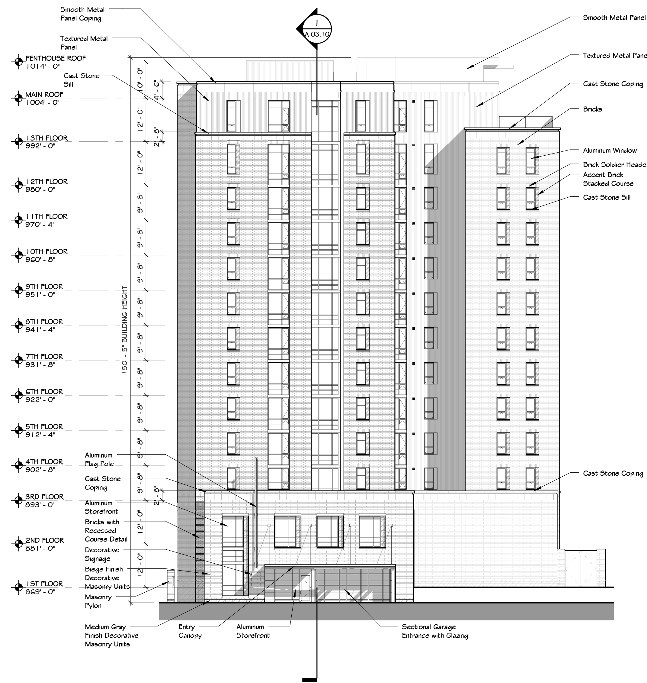
2 North Building Elevation Scale: 1/16" = 1'-0"
