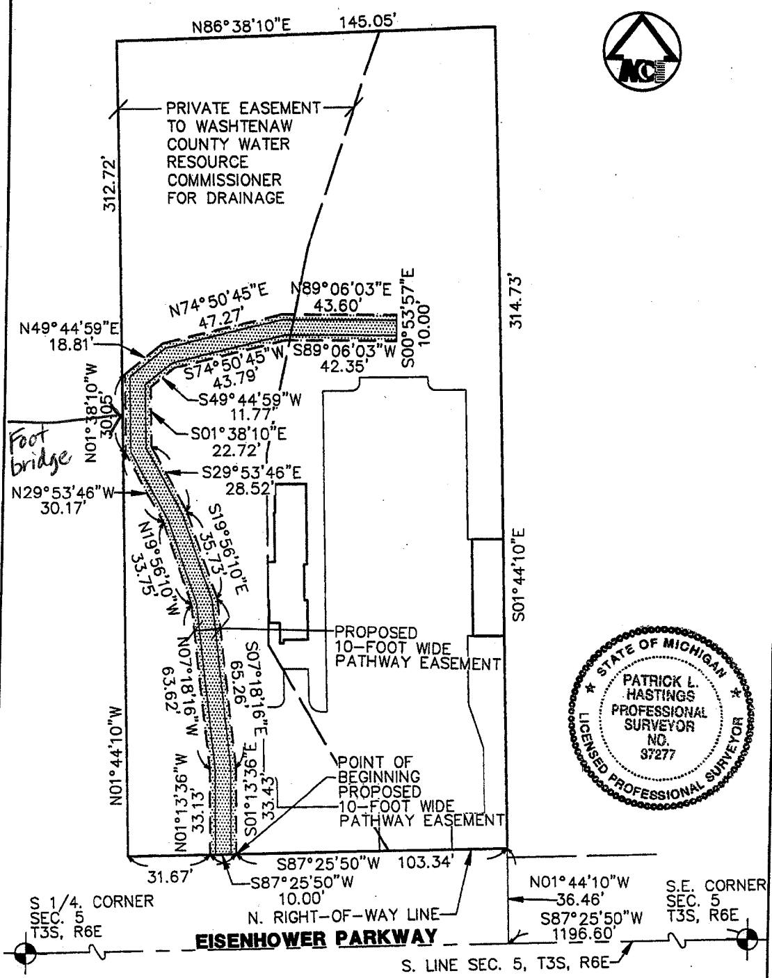
SKETCH OF A PROPOSED PATHWAY EASEMENT LOCATED IN THE SE 1/4 OF SECTION 5, T3S, R6E, CITY OF ANN ARBOR, WASHTENAW COUNTY, MICHIGAN
