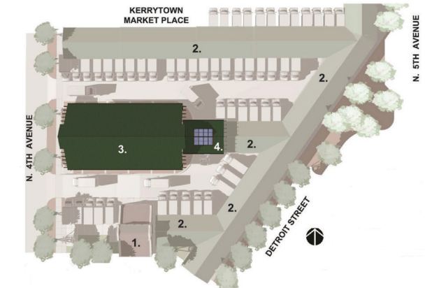
1. Existing Farmers Market building. 2. Existing vendor canopies. 3. New Farmers Market enclosures. 4. Drive-thru vendor canopy.
