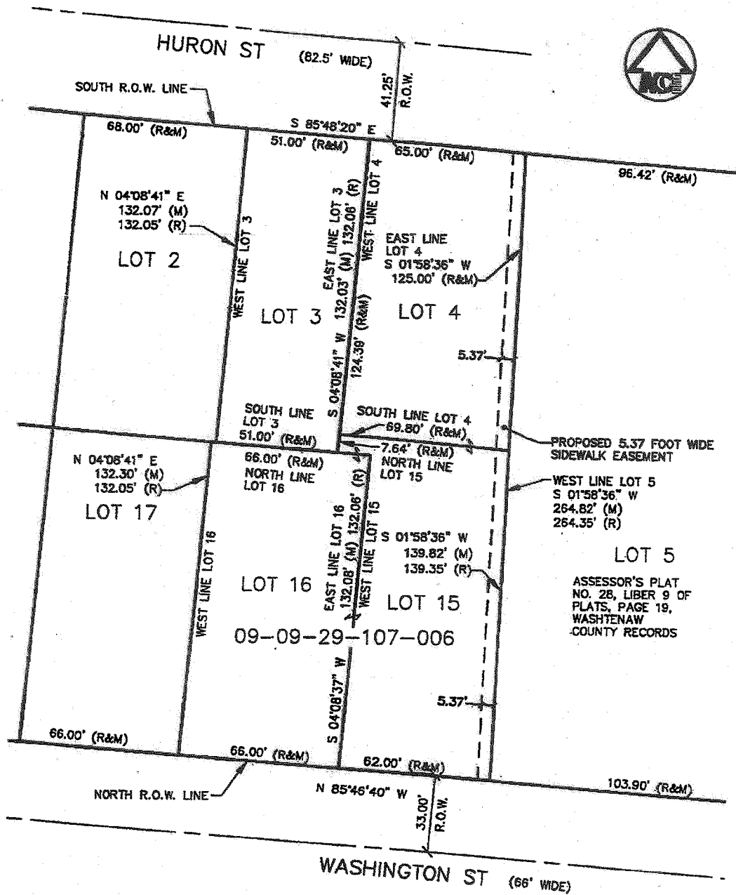
SKETCH OF A 5.37 FOOT WIDE SIDEWALK EASEMENT LOCATED IN SECTION 29, T2S, R6E, CITY OF ANN ARBOR, WASHTENAW COUNTY, MICHIGAN. REV: 1/23/13
