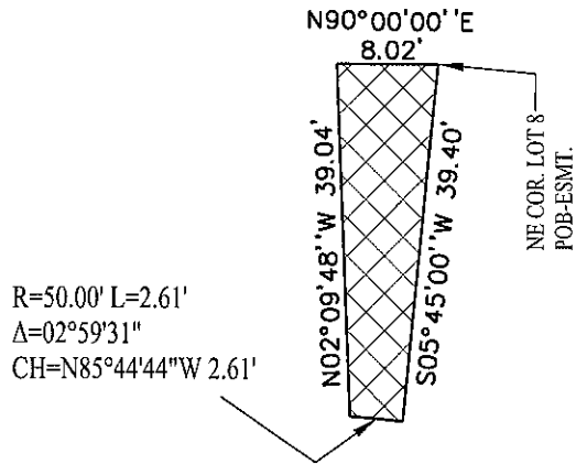
DETAIL - STORM SEWER EASEMENT (not to scale)
