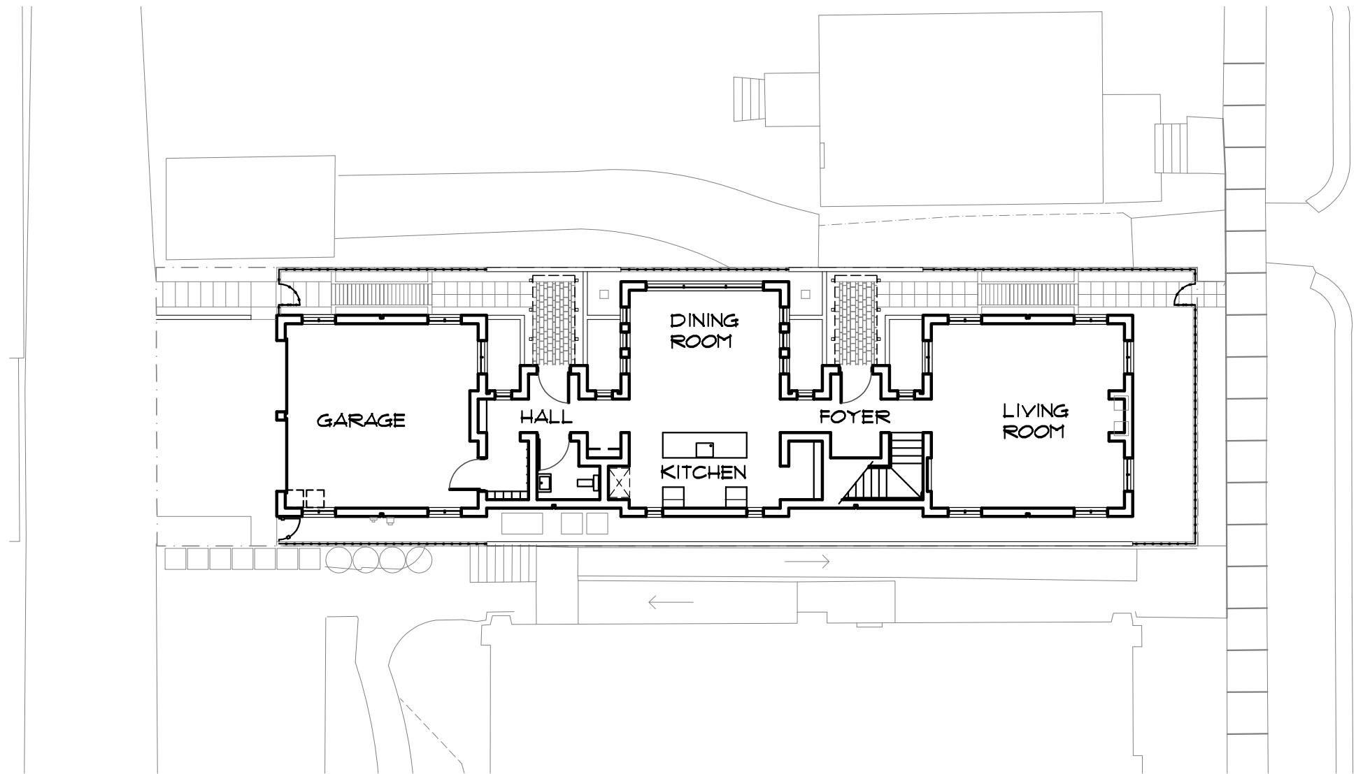
1 FLOOR PLAN A1.1 SCALE: 1/16" = 1'-0"
