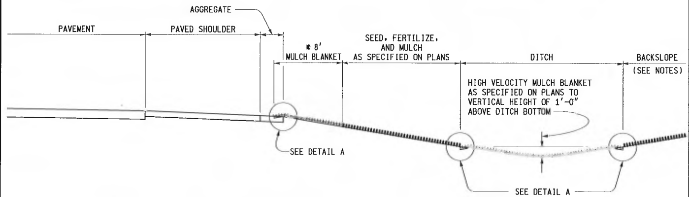
DETAIL A
