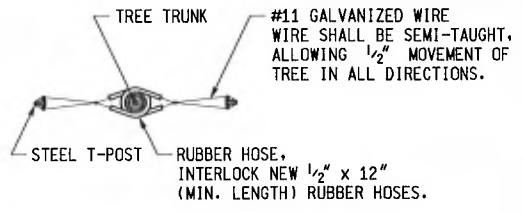
BRACING DETAIL
