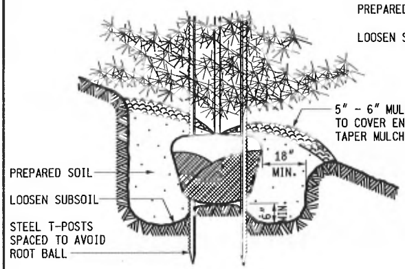
SLOPE PLANTING
