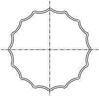
SECTION B-B 7 1/2" DIA. TAPERED 16 SHARP FLUTE N.T.S.
