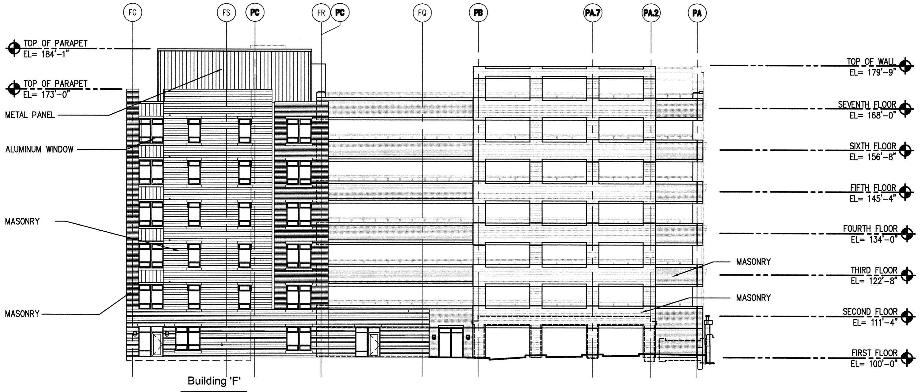
Parking Garage - South Elevation
